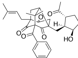
hyperberlone A
