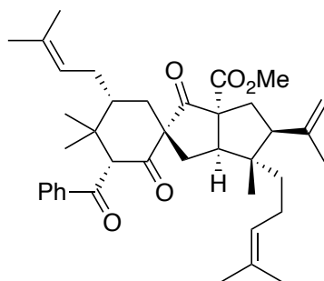
hyperbenzone A
